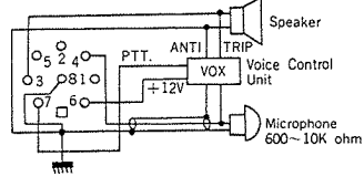
4. Headset or Telephoneset with VOX
