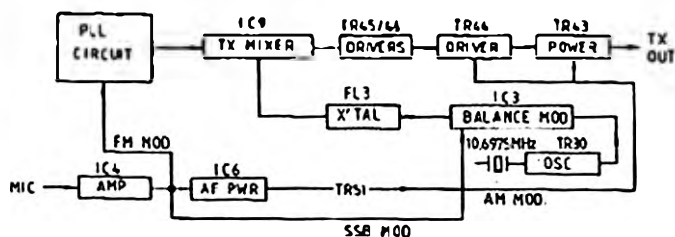
TRANSMITTER
