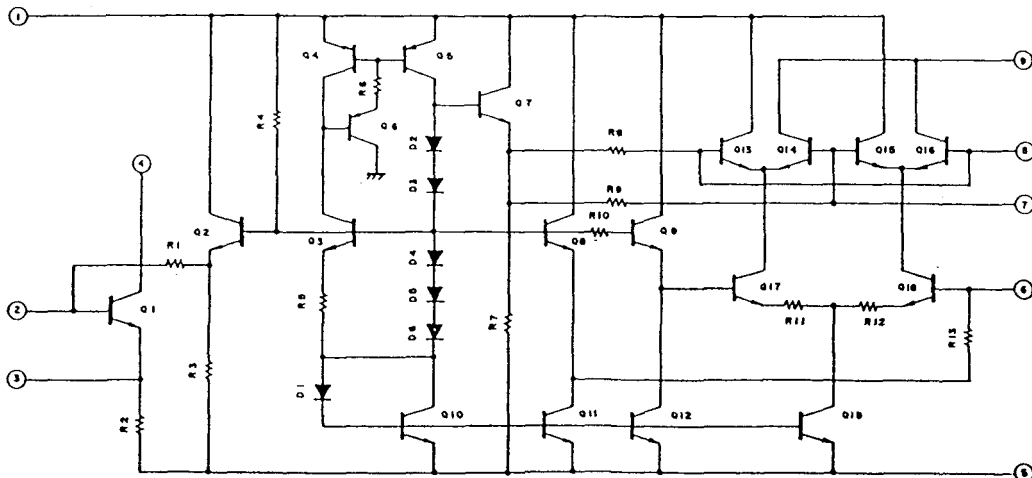
TA7320P BALANCED MODULATOR-DEMODULATOR
