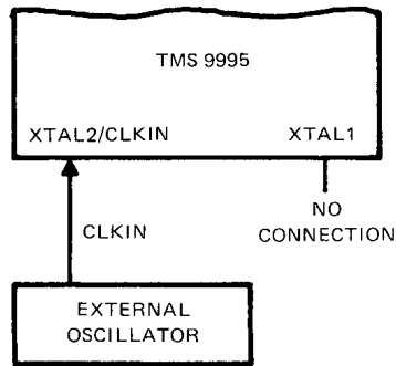
FIGURE 26 – EXTERNAL OSCILLATOR
