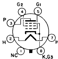
BOTTOM VIEW BASING DIAGRAM JEDEC TAC
