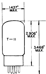
GLASS BULB SHORT INTERMEDIATE SHELL 7 PIN OCTAL A7-47 OUTLINE 11-1
