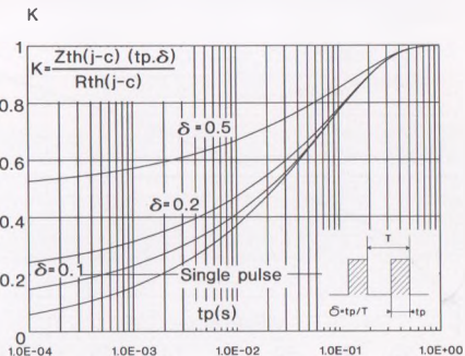
Fig 10 : Relative variation of thermal transient impedance junction to case versus pulse duration
