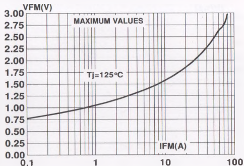
Fig 9 : Forward voltage drop versus forward current
