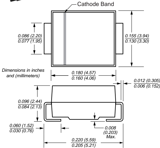
DO-214AA (SMB)
