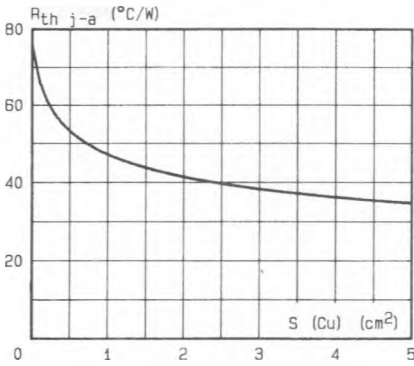
Fig.5 - Thermal resistance junction-ambient versus Cu surface (printed circuit).
