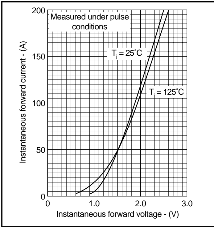
Fig.1 Maximum (limit) forward characteristics
