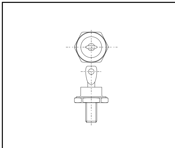
Outline type code: DO5. See Package Details for further information.
