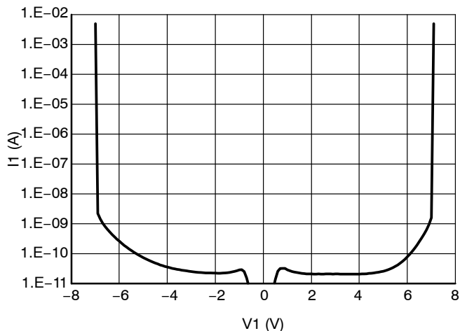
Figure 3. IV Characteristics
