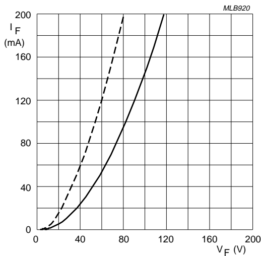
BY8110. Dotted line: T_j = 120\text{ }^\circ\text{C} . Solid line: T_j = 25\text{ }^\circ\text{C} .
