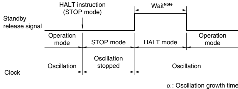
Figure 5-1. STOP Mode Release by Release Condition
