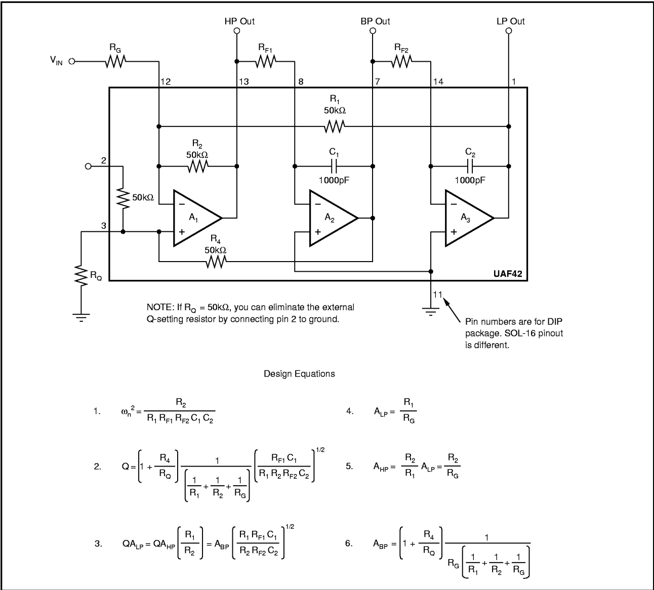
FIGURE 2. Inverting Pole-Pair.
