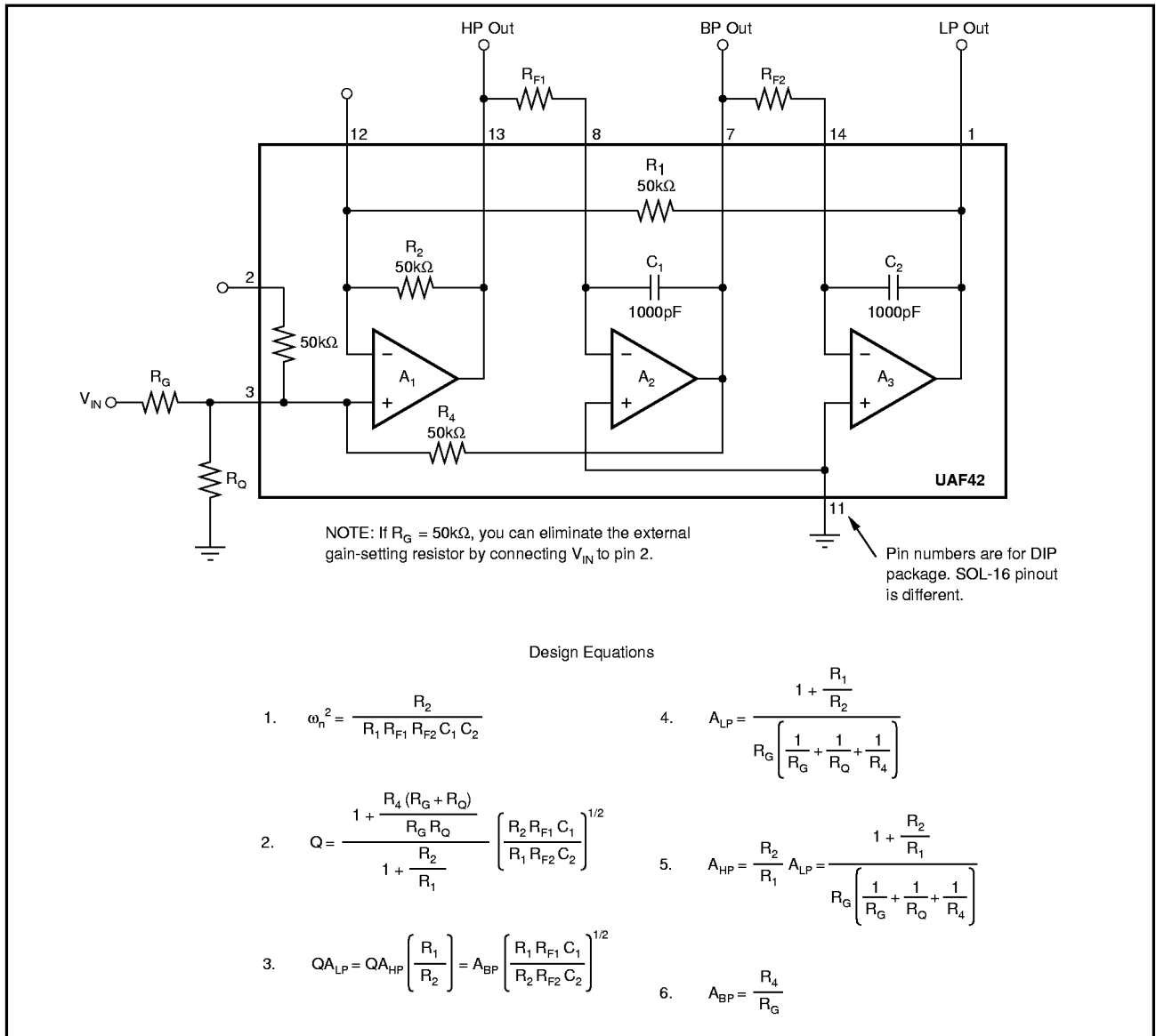
FIGURE 1. Non-Inverting Pole-Pair.
