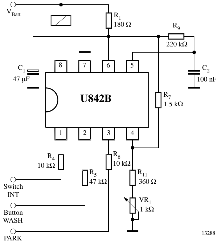
Figure 3. Basic circuitry
