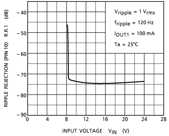
R.R.1 - V IN
