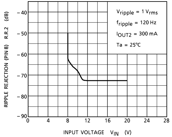
R.R.2 - V IN
