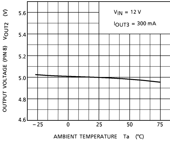
V OUT2 - T a
