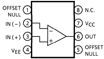
TA75071P
