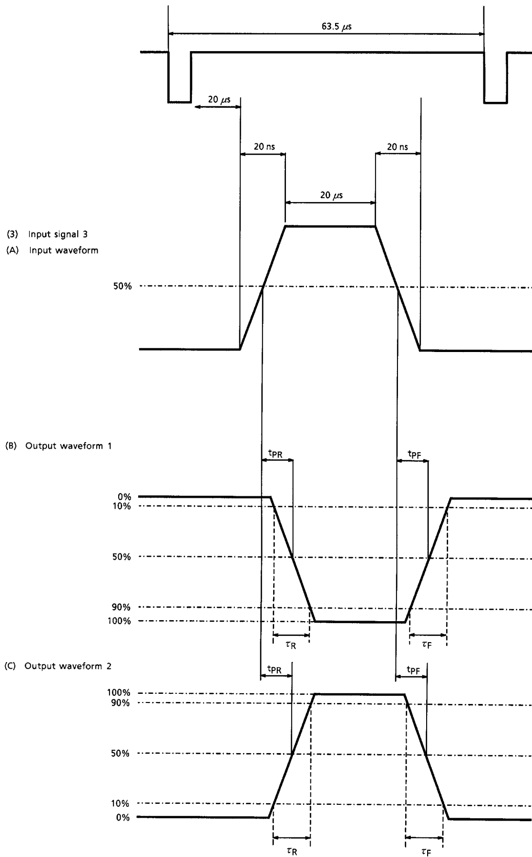
Fig.T-2 Test pulses for TA1310BN text stage
