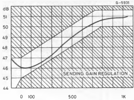
Figure 16 : Typical Gain Regulation with Line Length.
