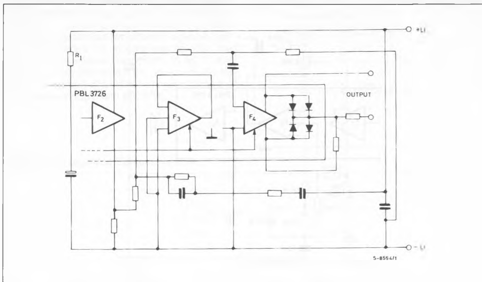
Figure 26 : Wheatstone Type Sidetone Network.
