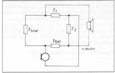
Figure 23 : Balance Bridge.
