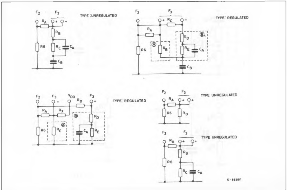
Figure 7 : Sidetone Network.
