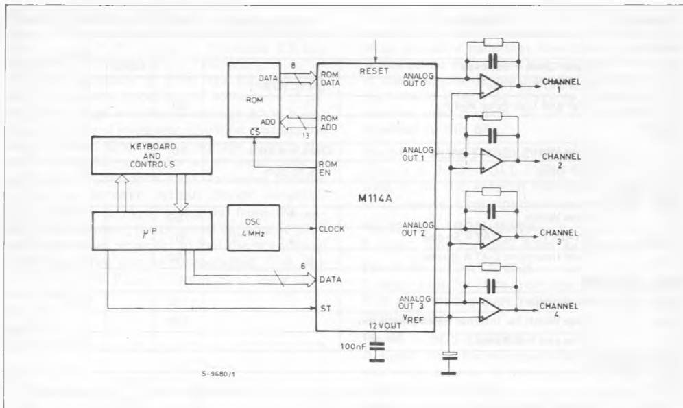
Fig. 2 – System Configuration
