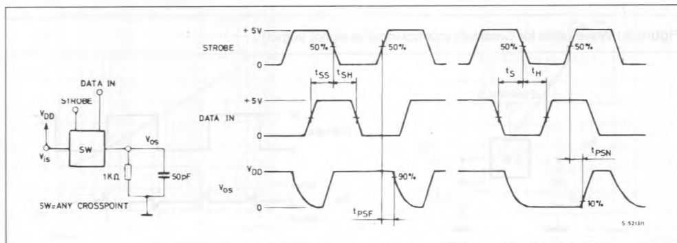
Figure 6 : Propagation Delay Time and Waveforms (data-in signal output, switch Turn-ON to high or low level).
