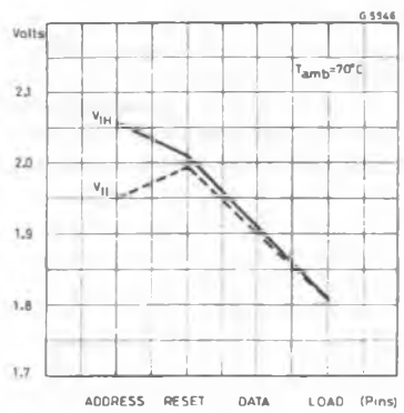
Pin Dependence V IH and V IL .
