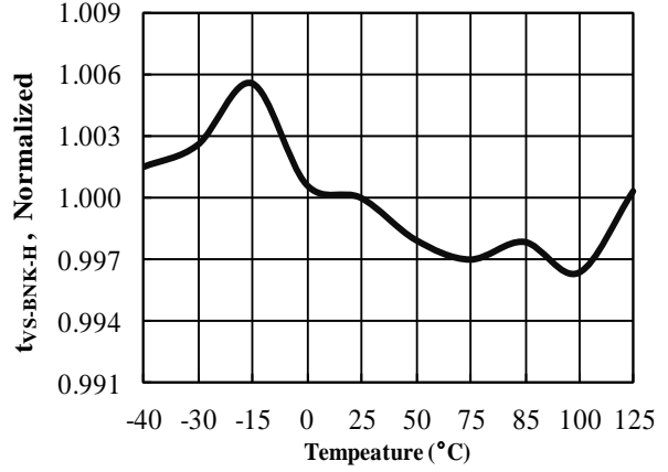
Figure 10. Vs Sampling Blanking Time ( t_{VS-BNK-H} ) vs. Temperature
