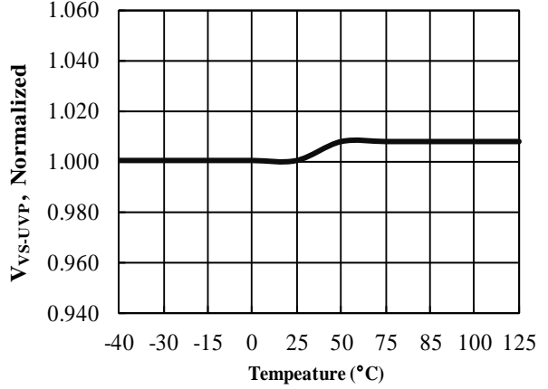
Figure 12. Output Under-Voltage of Vs sampling Threshold ( V_{VS-UV} ) vs. Temperature
