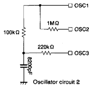
Oscillator circuit 2
