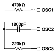
Oscillator circuit 1
