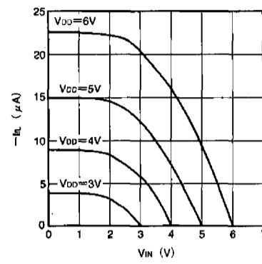
Fig. 16 RESETB and SETB pins: pull-up resistance characteristic
