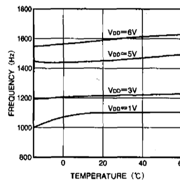
Fig. 10 Oscillation frequency - temperature characteristic (circuit 2)
