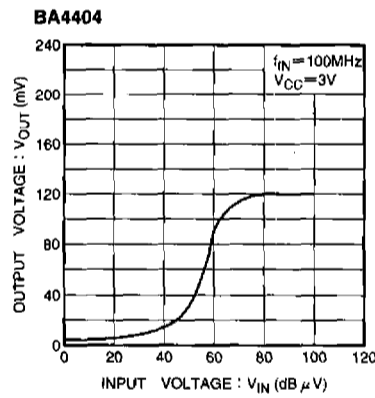
Fig. 9 Output voltage vs. input voltage
