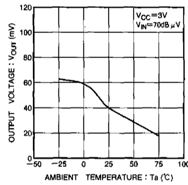
Fig. 8 Output voltage vs. ambient temperature
