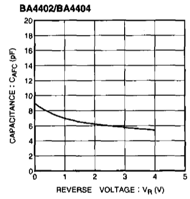
Fig. 15 AFC capacitor capacitance vs. applied voltage
