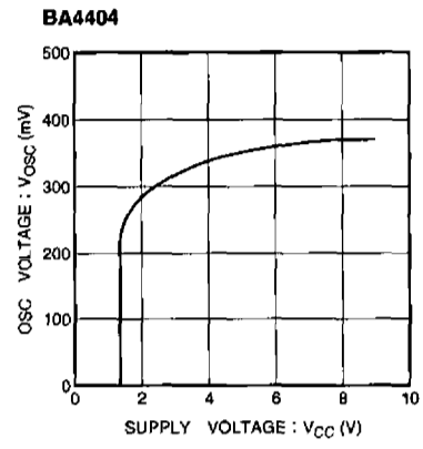
Fig. 12 Oscillator voltage vs. supply voltage
