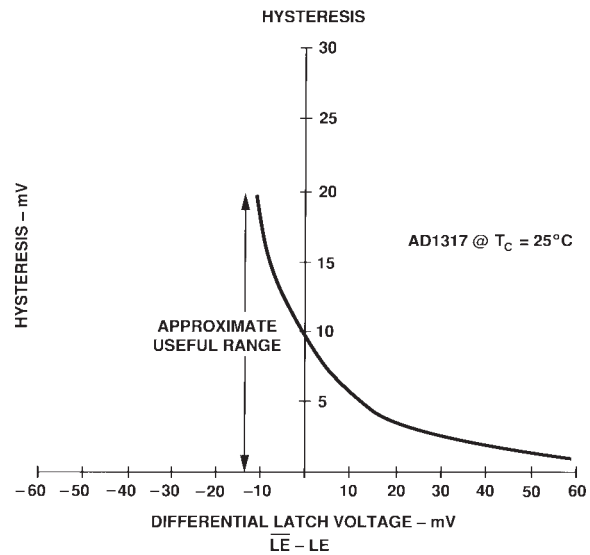
Figure 29. Typical Hysteresis Curve
