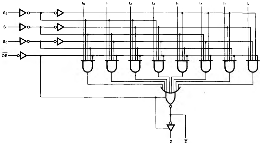
LOGIC DIAGRAM
