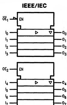
TL/F/10659-1
