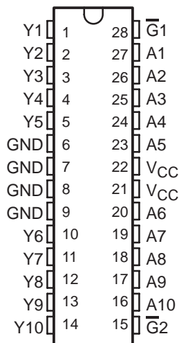
DW OR NT PACKAGE (TOP VIEW)
