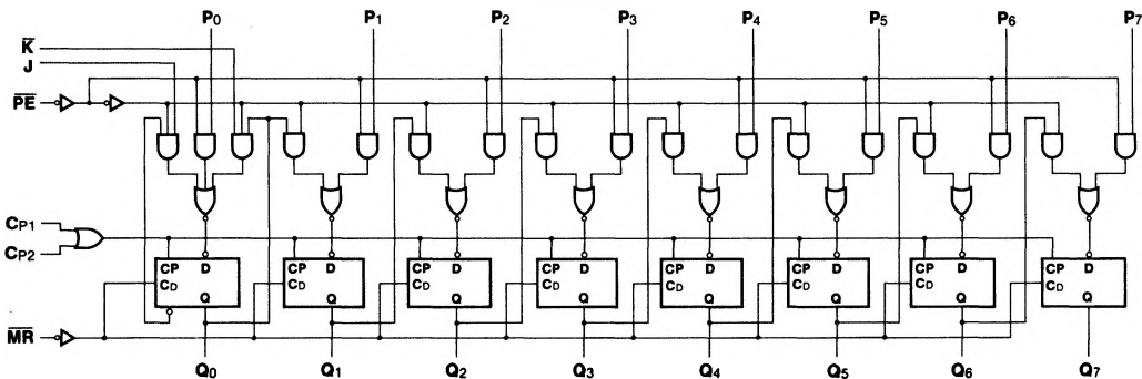
LOGIC DIAGRAM
