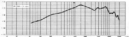
Nominal frequency response
